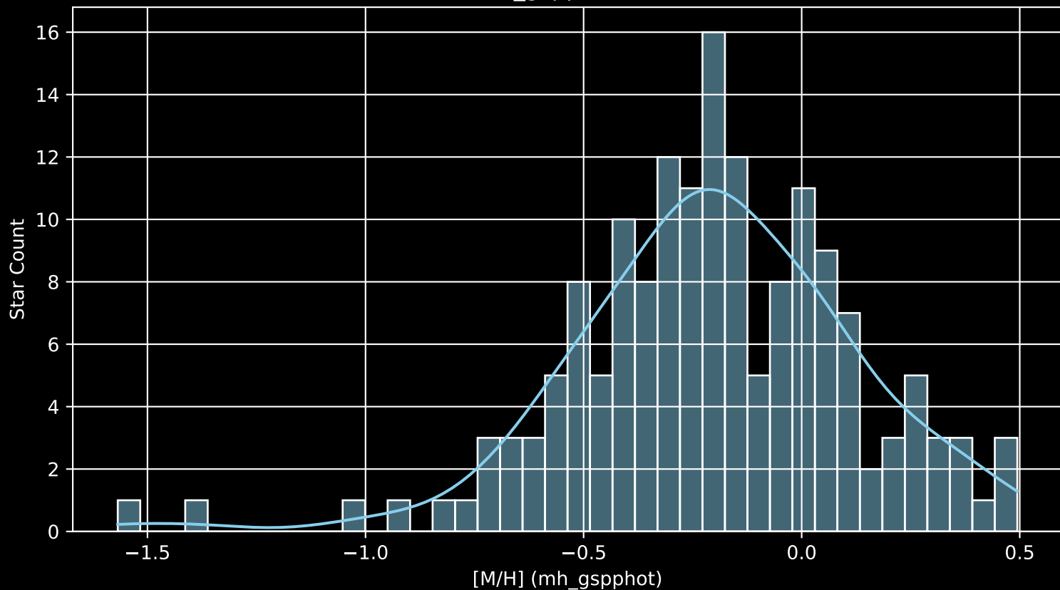
APOGEE DR17 Field: [054+87_MGA [M/H] (mh_gspphot) (n= 162)
