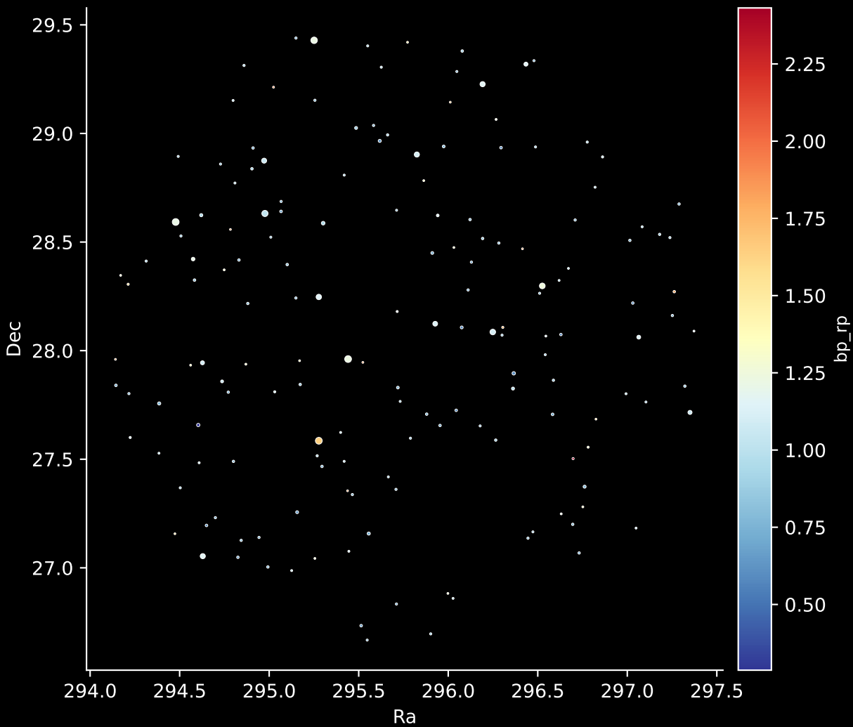
APOGEE DR17 Field: [054+87_MGA] Stars: 164
