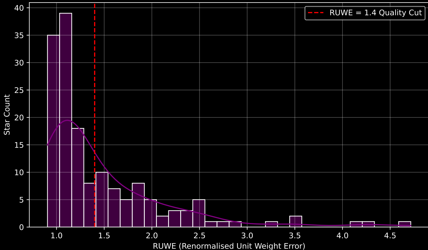
GAPOGEE DR17 Field [054+87_MGA] RUWE Distribution (n= 157)
