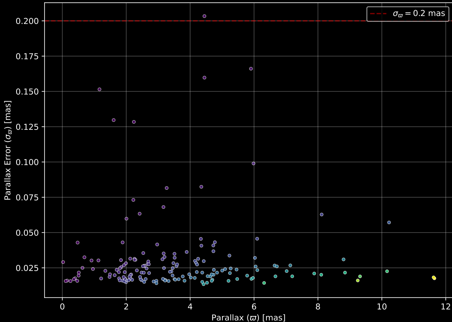
APOGEE DR17 Field: [054+87_MGA] Parallax Quality (n= 164)
