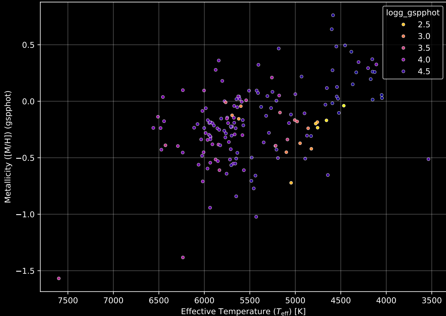
APOGEE DR17 Field: [054+87_MGA] Stellar Population Parameters (n= 164)
