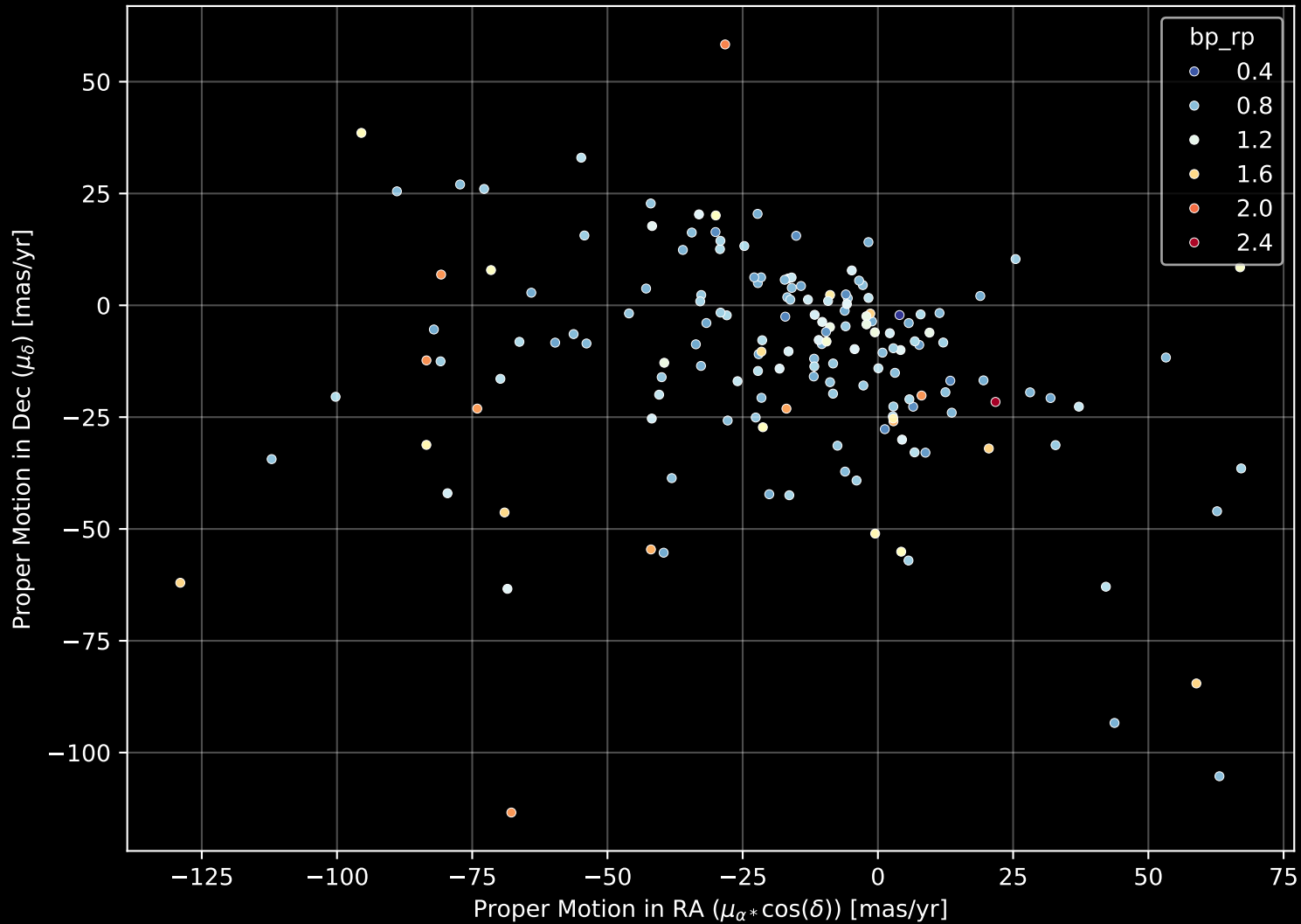
APOGEE DR17 Field: [054+87_MGA] Proper Motion Diagram (n= 164)
