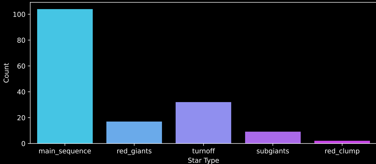
APOGEE DR17 Field: [054+87_MGA] Count plot of Star Type
